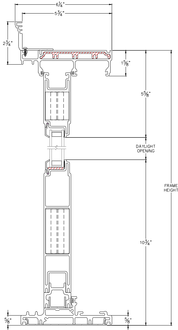
HEAD & SILL
