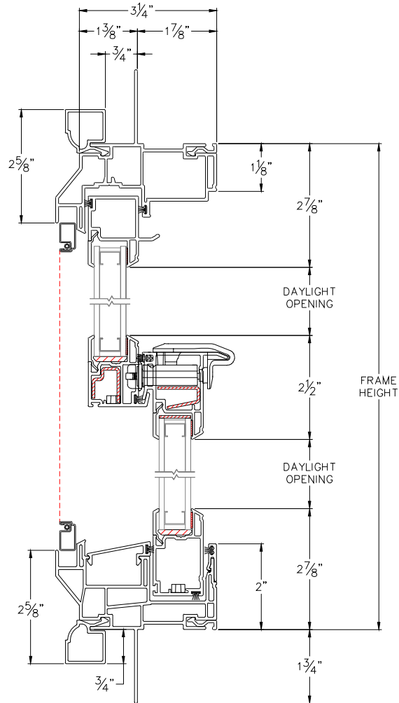
HEAD & SILL
